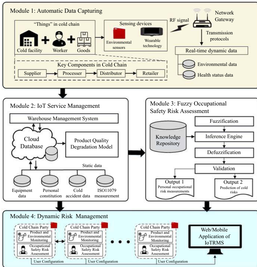
Figure 2. System architecture of IoTRMS
