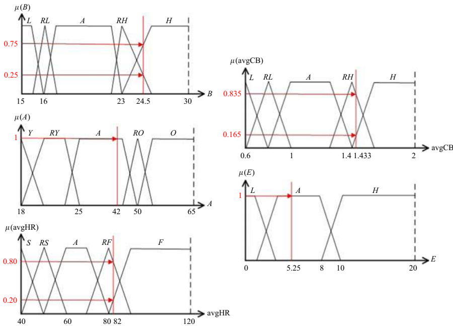
IoT-based risk monitoring system
