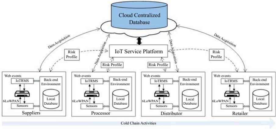
Figure 11. Information flow of IoTRMS in cold chain
